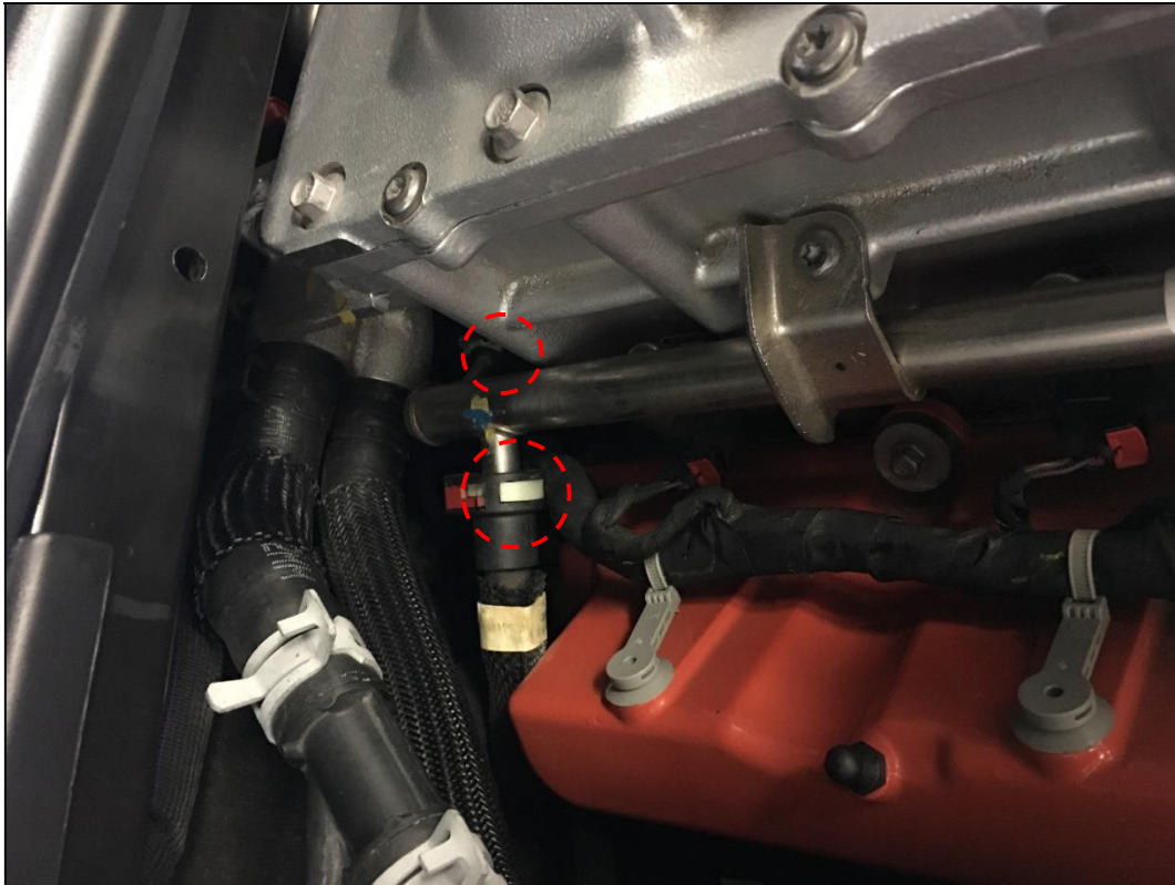
Figure 13 – Fuel line removal
