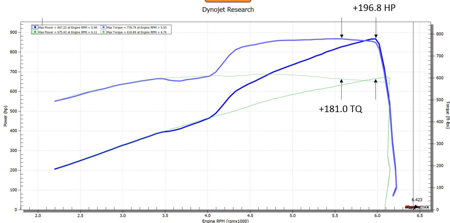
Figure 21 – Dyno Graph
