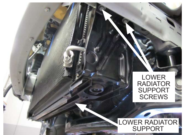
Fig. 2-u: Remove lower radiator support hardware
