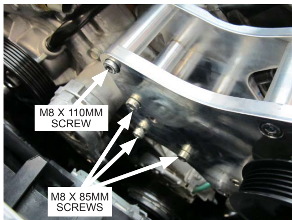
Fig. 5-g: Secure S/C mounting bracket hardware
