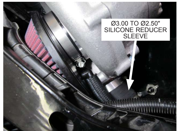
Fig. 7-h: Secure air filter and discharge tube A to supercharger
