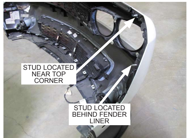
Fig. 2-h: Remove two nuts (Bumper removed for clarity)
