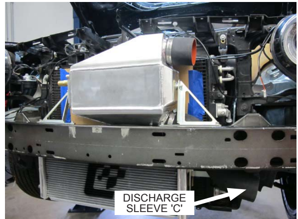
Fig. 6-v: Install air/water cooler
