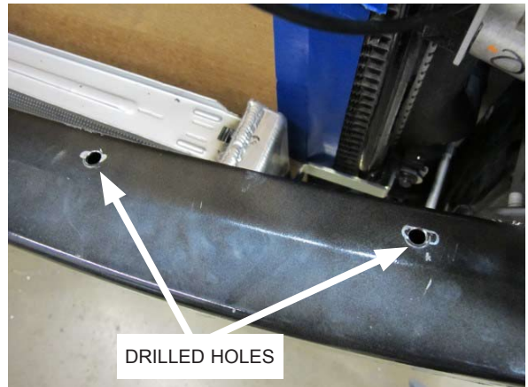
Fig. 6-s: Drill 2x holes using 6" length drill bit
