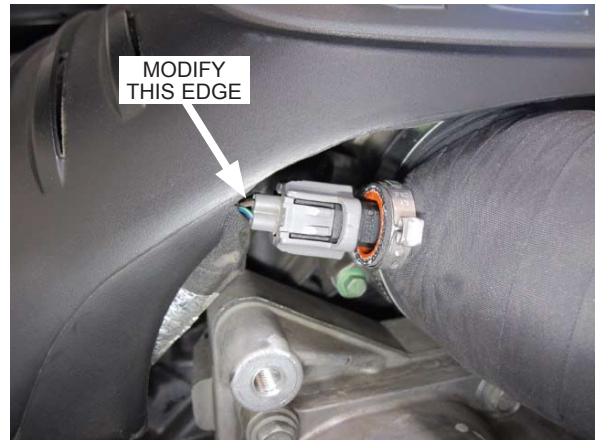
Fig. 10-d: Modify passenger side engine cover
