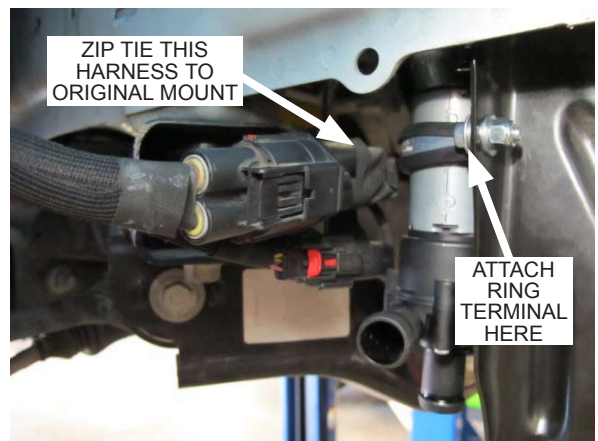
Fig. 8-f: Install the auxiliary water pump
