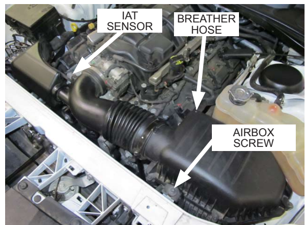
Fig. 2-r: Remove airbox and air inlet duct
