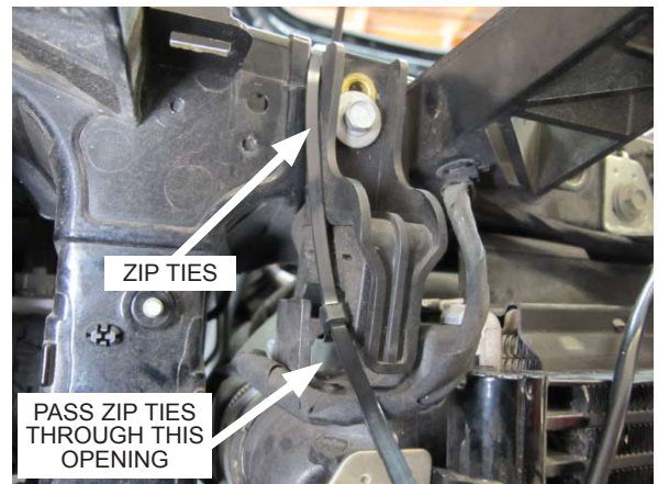
Fig. 2-t: Zip tie radiator to core support
