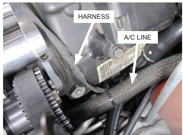
Fig. 5-k: Secure harness to A/C line
