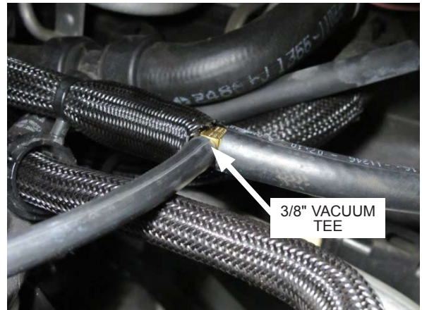
Fig. 7-j: Install vacuum tee
