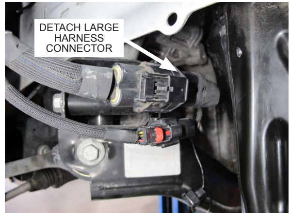
Fig. 8-d: Large harness connector
