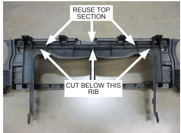
Fig. 9-d: Modify radiator shroud
