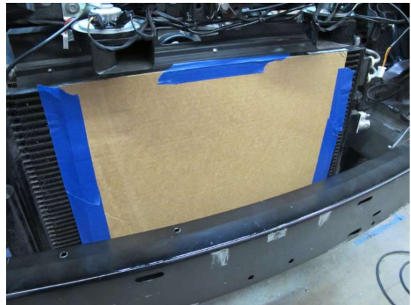
Fig. 6-b: Cover A/C condenser with cardboard
