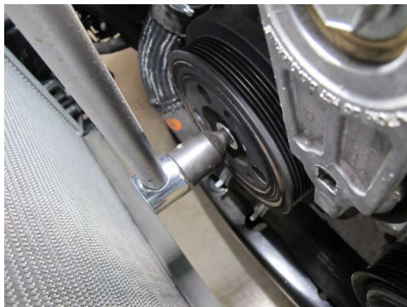
Fig. 3-a: Remove crankshaft damper bolt
