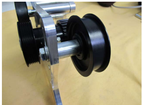
Fig. 5-c: Remove cog belt idler pulley
