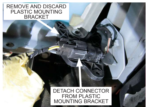
Fig. 2-i: Disconnect fog light connector
