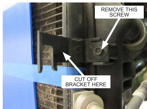
Fig. 6-c: Remove aluminum bracket and screw
