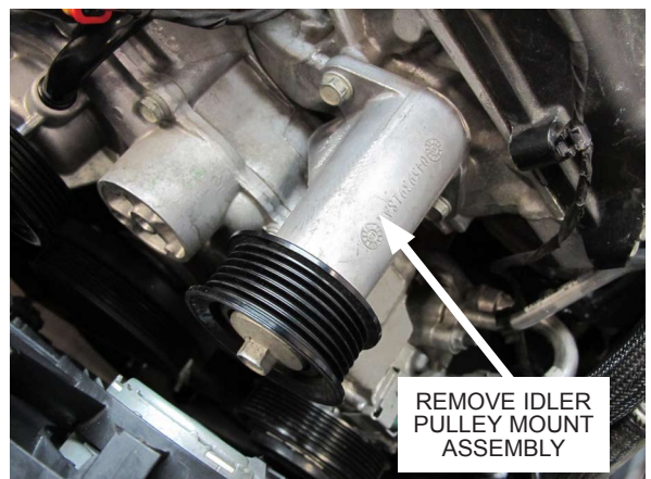
Fig. 2-x: Remove idler pulley mount assembly
