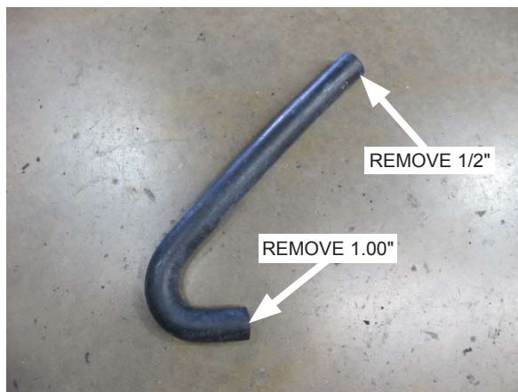
Fig. 8-i: Modify 150° molded hose as shown
