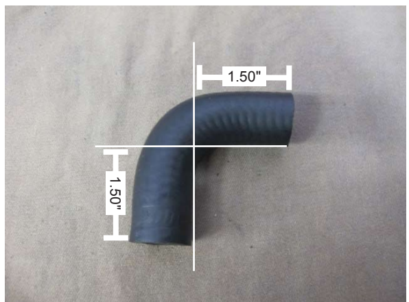
Fig. 8-o: Modify 1/2" x 90° coolant elbow as shown
