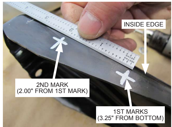
Fig. 4-e: Measure 2.00" up from first marks
