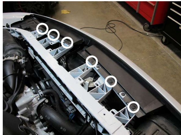
Fig. 2-b: Remove six plastic fasteners
