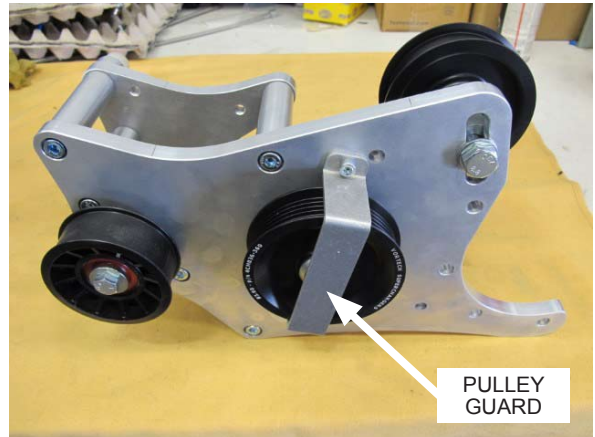
Fig. 5-a: Remove pulley guard
