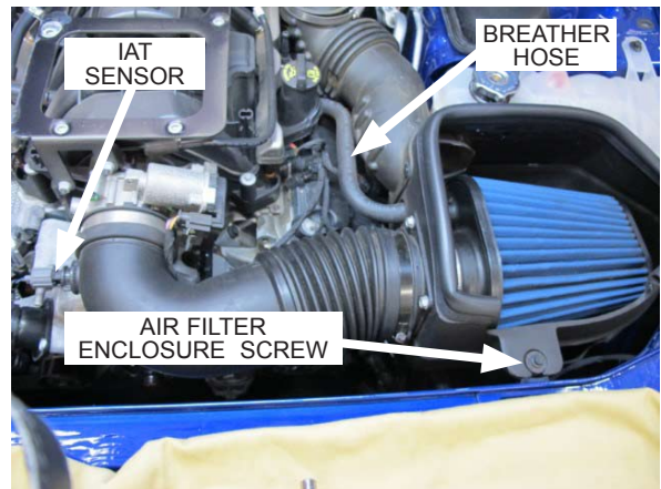
Fig. 2-q: Shaker inlet removal
