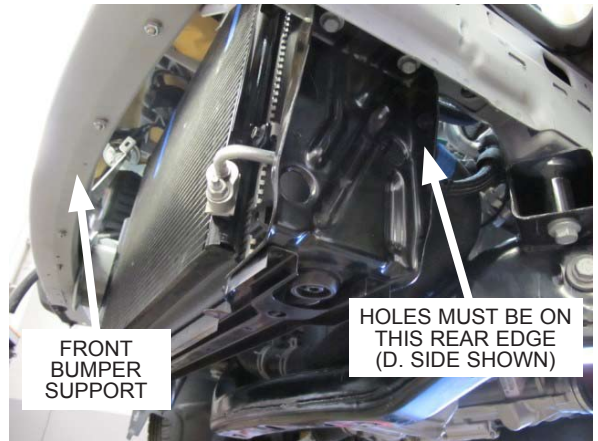
Fig. 4-h: Reinstall lower radiator support
