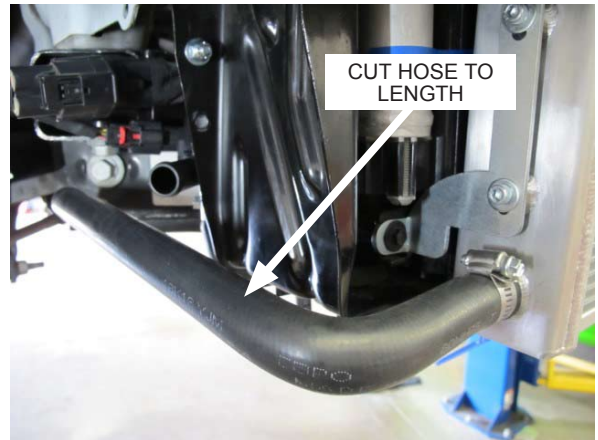
Fig. 8-v: Install 3/4" x 90° hose
