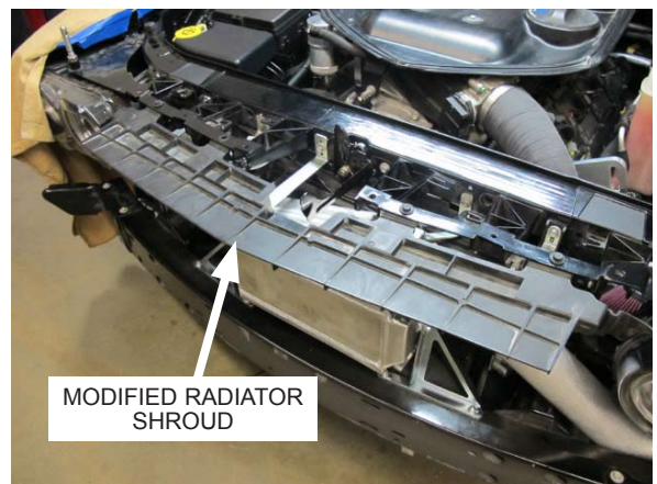
Fig. 9-f: Secure modified radiator shroud and three radiator shroud brackets
