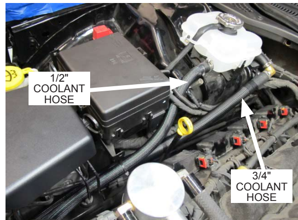
Fig. 8-y: Install coolant hose assembly and route towards electric water pump
