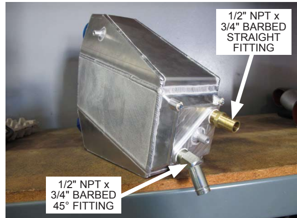
Fig. 6-a: Install fittings to air/water cooler
