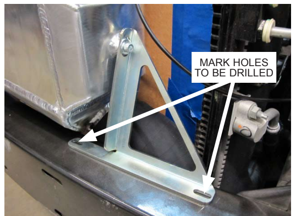
Fig. 6-r: Use driver side air/water cooler support bracket as drill template
